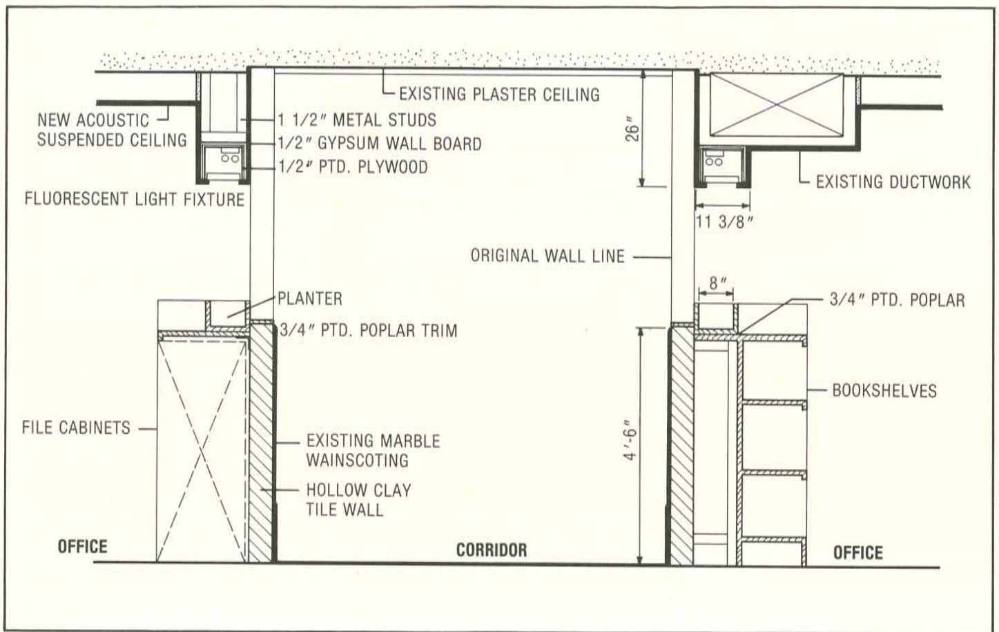
Figure 3. The innovative rehabilitation solution involved removing sections of wall above the marble wainscoting, leaving the historic door frames and transoms in place, and constructing soffits above. Drawing: Chris Henry.
